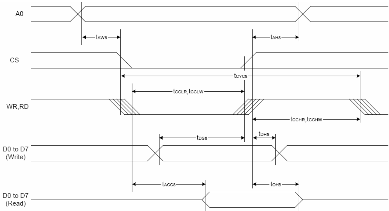
System Bus Read/Write Characteristics (For the 8080 Series MPU)
