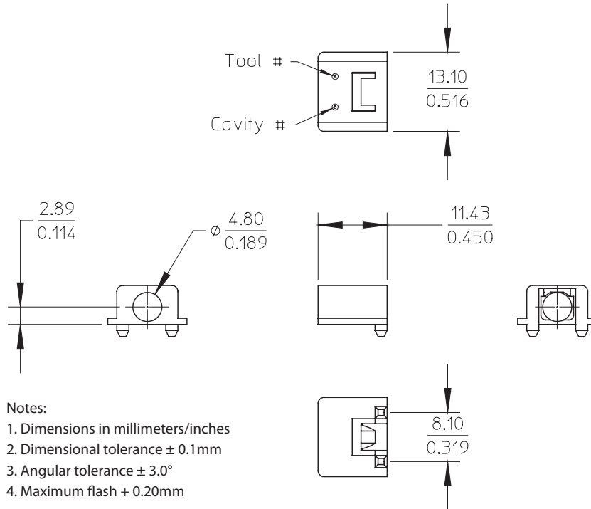
Figure 1. ADNS-5200 Solid State Optical Mouse LED Assembly Clip outline drawing and detail
