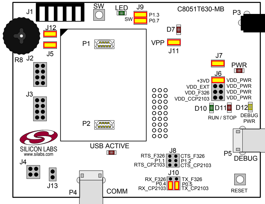
Figure 4. C8051T630 Motherboard Default Shorting Block Positions
