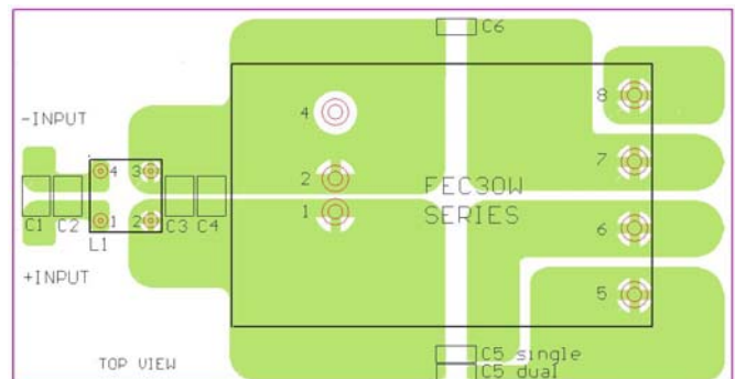
Recommended EN55022 Class B Filter Circuit Layout
