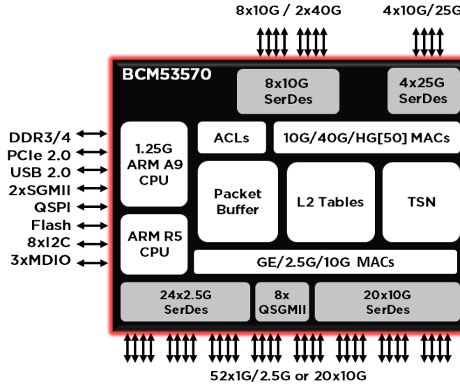
BCM53570 Block Diagram
