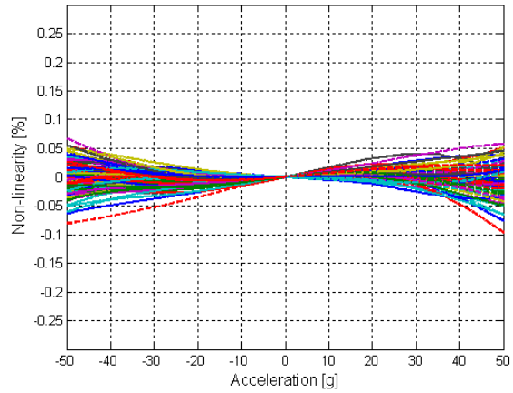
Figure 13 : Non linearity under vibration
