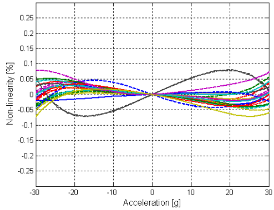
Figure 9 : Non linearity under vibration
