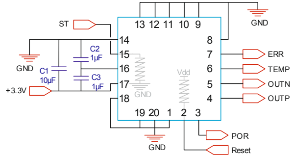
Figure 2: Proximity circuit & pull-up/down
