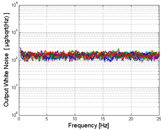
Figure 14: typical white noise
