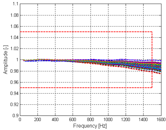
Figure 12: Typical frequency response
