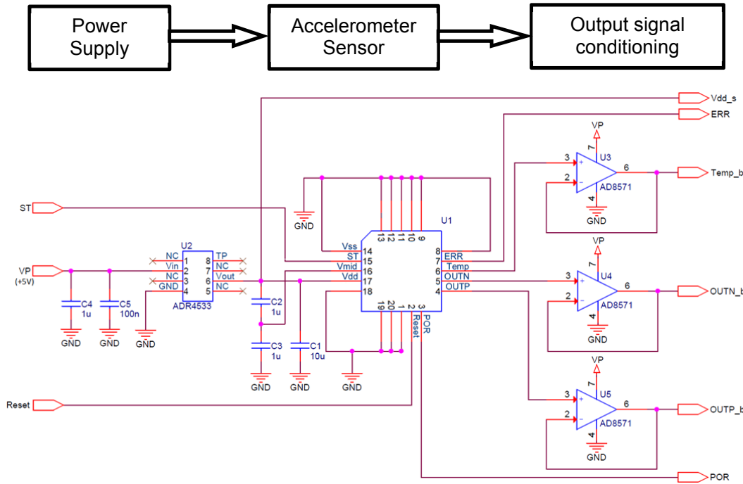
Figure 20: Recommended circuit
