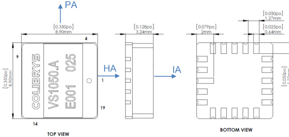
Figure 7: Package mechanical dimension
