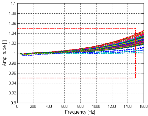
Figure 8: Typical frequency response
