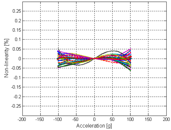
Figure 17 : Non linearity under vibration
