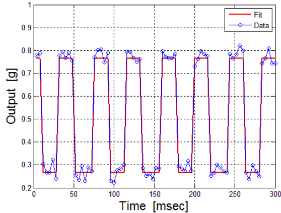
Figure 5: Built-in Self-test signal on the differential acceleration output (frequency: 24 Hz / amplitude 0.5 g)
