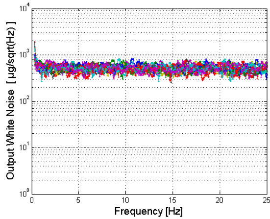
Figure 18: typical white noise
