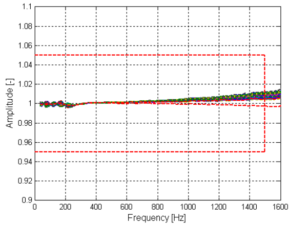
Figure 16: Typical frequency response
