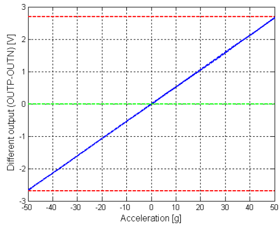
Figure 15: Differential acceleration output (OUTP-OUTN) at full scale
