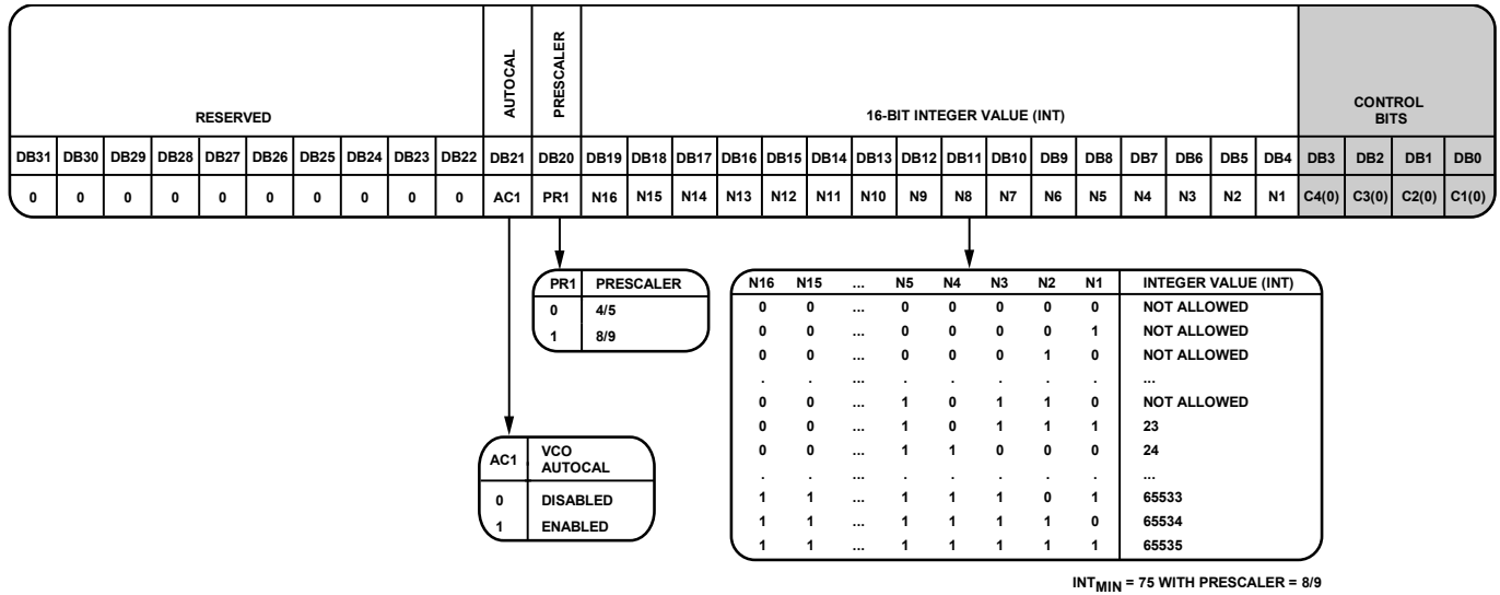
Figure 41. Register 0
