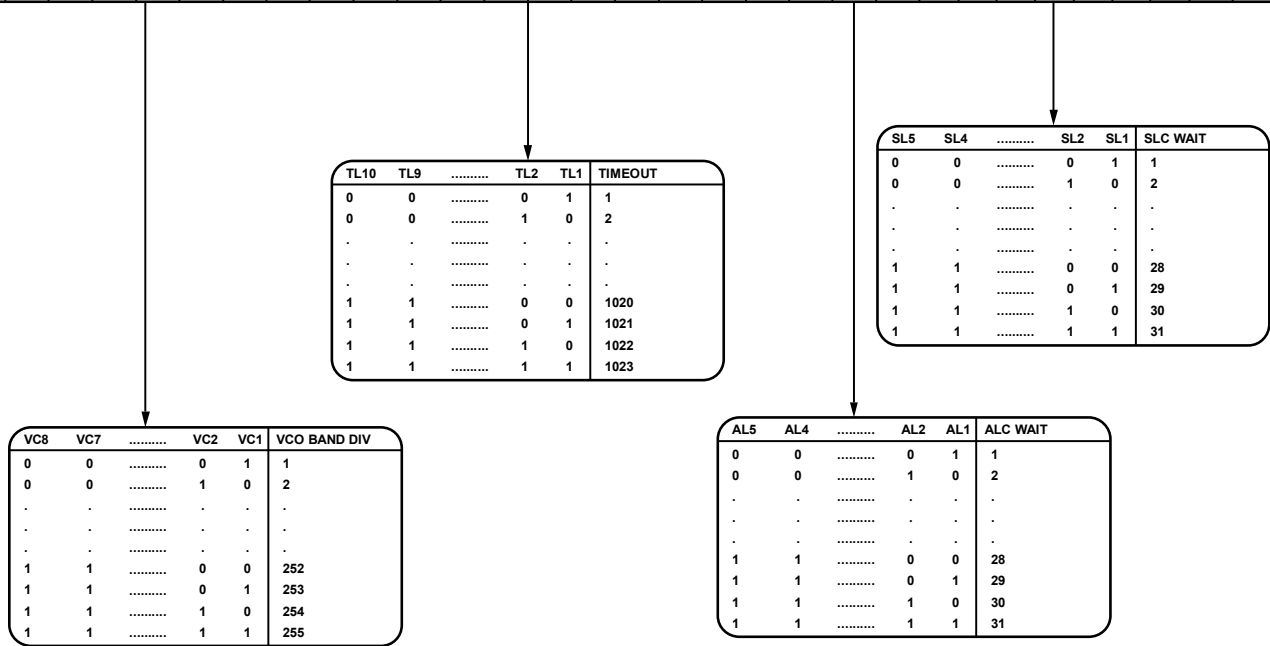
Figure 50. Register 9
