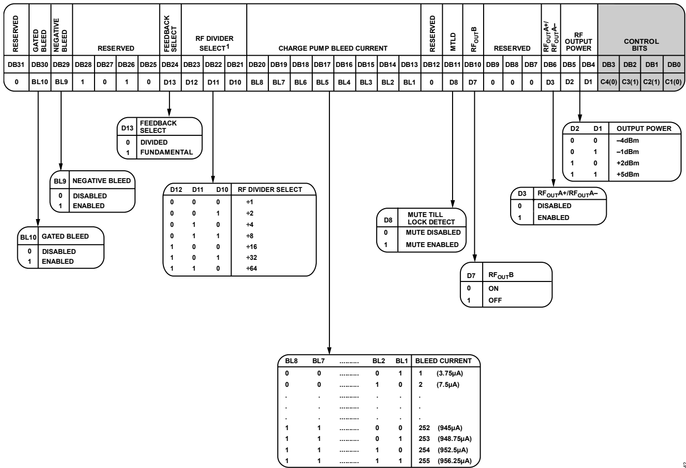
Figure 47. Register 6
