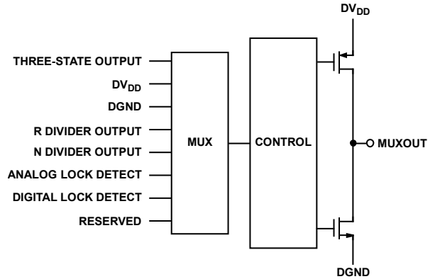
Figure 35. MUXOUT Schematic
