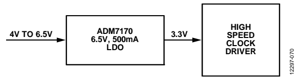
Figure 67. Clock Driver
