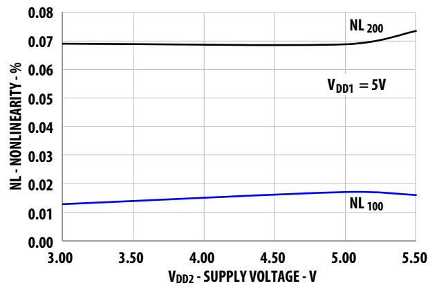
Figure 10. Nonlinearity vs. supply V_{DD1}
