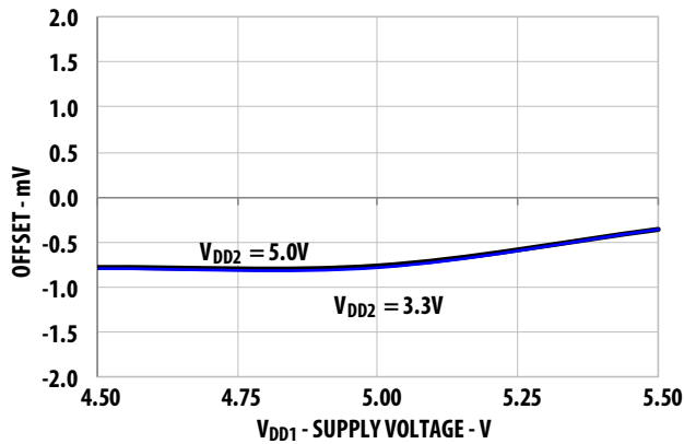
Figure 3. Input offset vs. supply V_{DD1}
