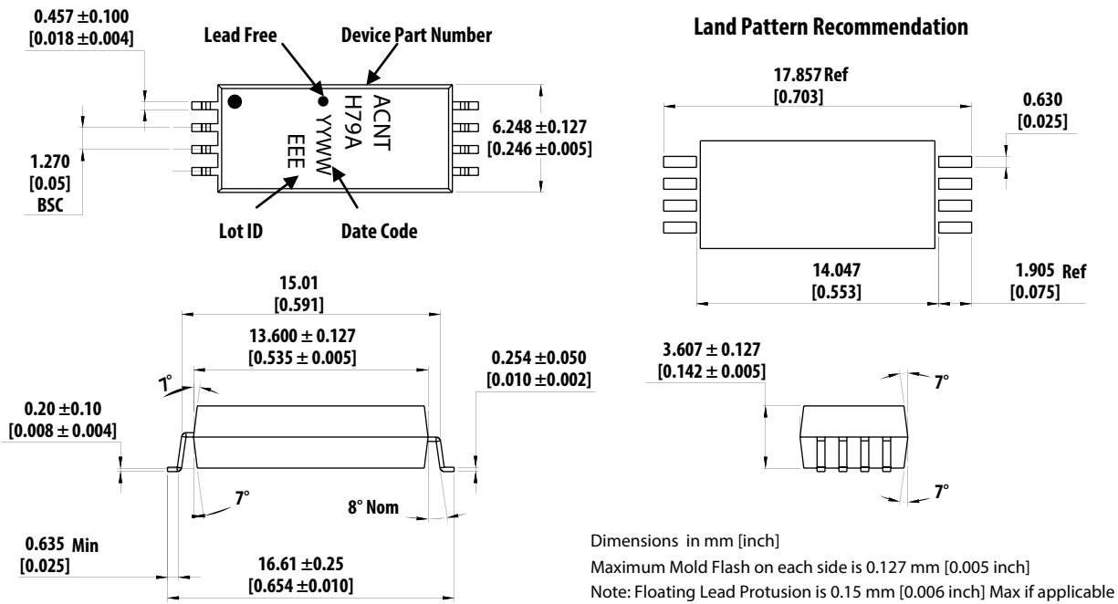
Figure 2. 14.2mm SO-8 Package
