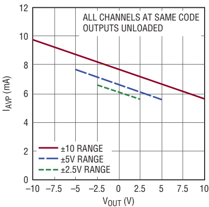
AVP Supply Current vs Bipolar Output Voltage
