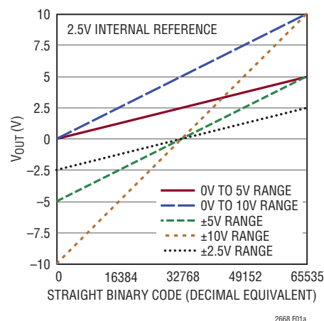
Figure 2a. LTC2668-16 Transfer Function
