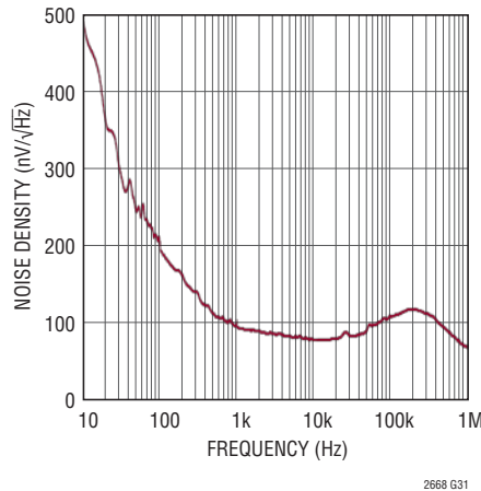
Noise Density vs Frequency
