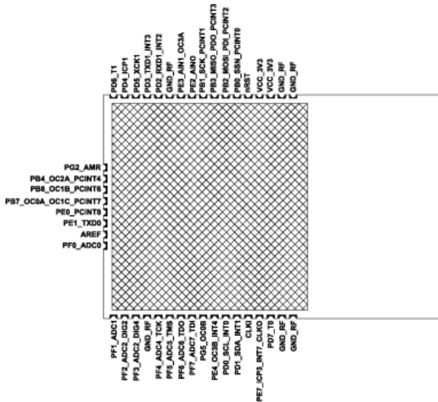
Figure 3-2. ATZB-S1-256-3-0-C Pinout
