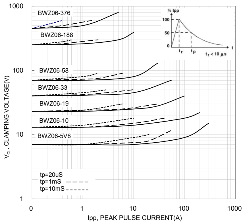
FIG. 4 CLAMPING VOLTAGE CURVE
