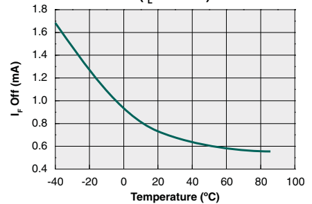
Typical I_F for Switch Dropout vs. Temperature ( I_L=250\text{mA} )
