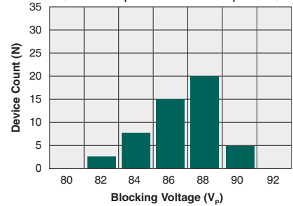
Typical Blocking Voltage Distribution (N=50, T_A=25^\circ\text{C} ) (Form-A I_F=0\text{mA} , Form-B I_F=2\text{mA} )
