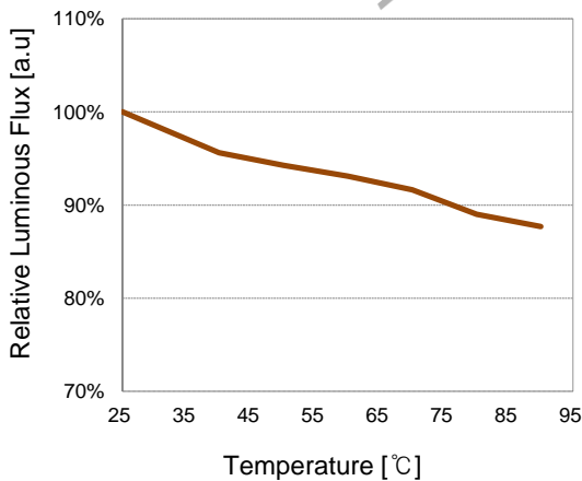
■ Luminous Flux vs. Temp.
