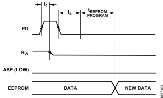
Figure 4. Auto Save Mode Timing
