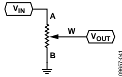
Figure 43. Potentiometer Mode Configuration
