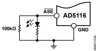
Figure 40. Typical End Scale Indicator Circuit
