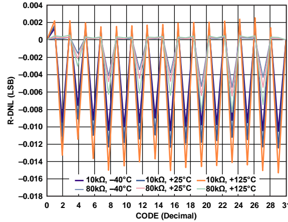
Figure 11. R-DNL vs. Code (AD5115)
