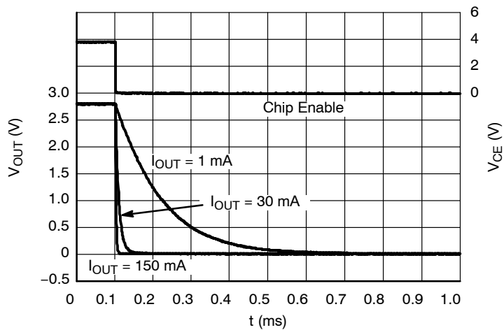
Figure 57. Shutdown, NCP4682 2.8 V Version H, V_{IN} = 3.8 V
