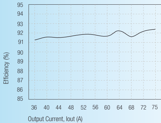
Input Without Heatsink RP100-4805SB
