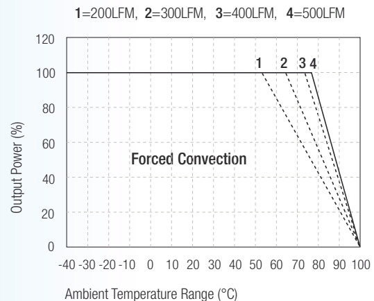
Input With Heatsink (7G-0022) RP100-4805SB
