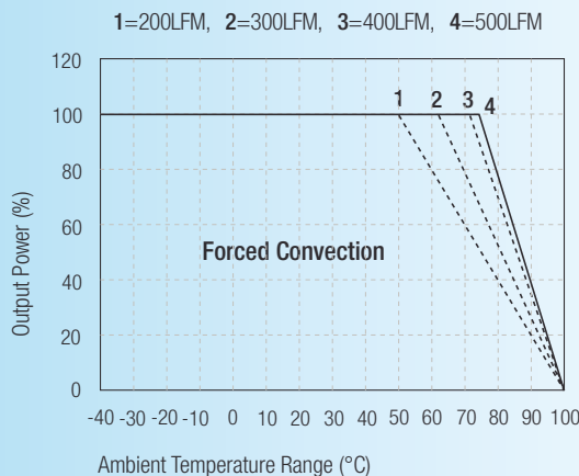
Input Without Heatsink RP100-4805SB
