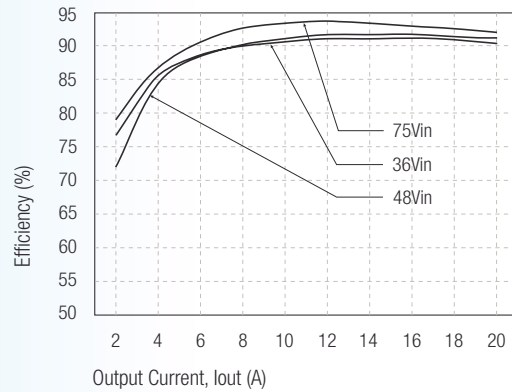
Input With Heatsink (7G-0022) RP100-4805SB
