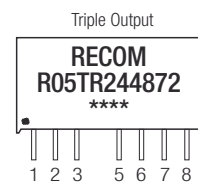
Pin Connections
