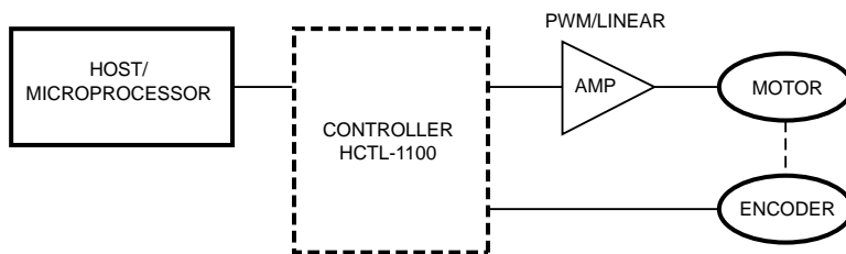
Figure 1. Closed Loop Position and Velocity Control of DC Brush Motor
