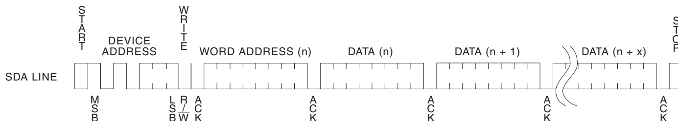
Figure 5-2. Page Write
