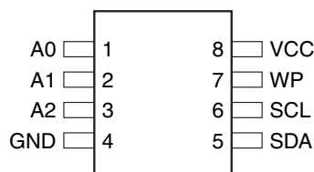
8-lead SOIC
