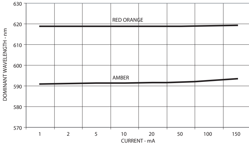
Figure 7. Dominant Wavelength Vs. Forward Current - AllnGaP Devices
