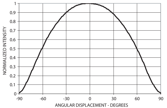
Figure 9. Radiation Pattern
