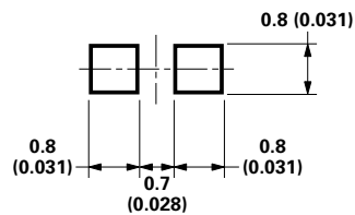
Figure 10. Recommended soldering pattern for HSMx-C190 and HSMx-C191.
