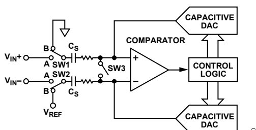
Figure 26. ADC Differential Configuration During Conversion Phase
