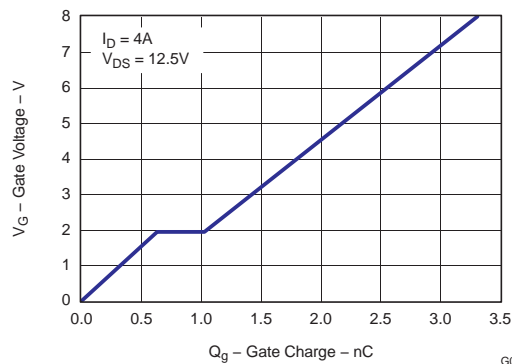
GATE CHARGE
