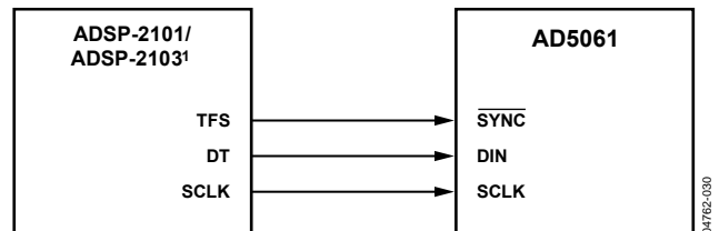
Figure 40. AD5061-to-ADSP-2101/ADSP-2103 Interface
