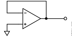
Figure 59. Configuration for Unused Amplifiers
