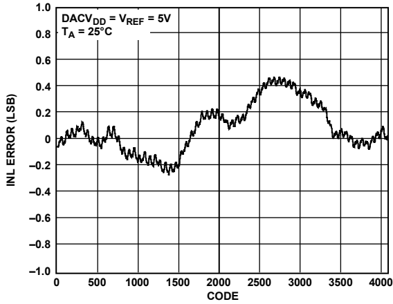
Figure 6. DAC INL, External Reference
