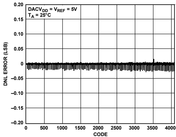
Figure 7. DAC DNL, External Reference
