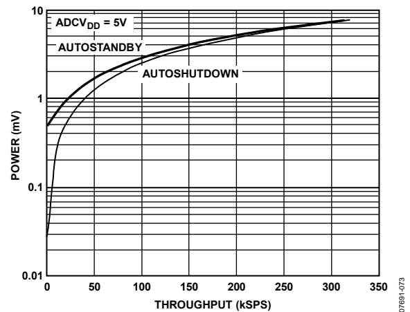
Figure 73. Power vs. Throughput Rate in Autoshtutdown and Autostandby Mode
