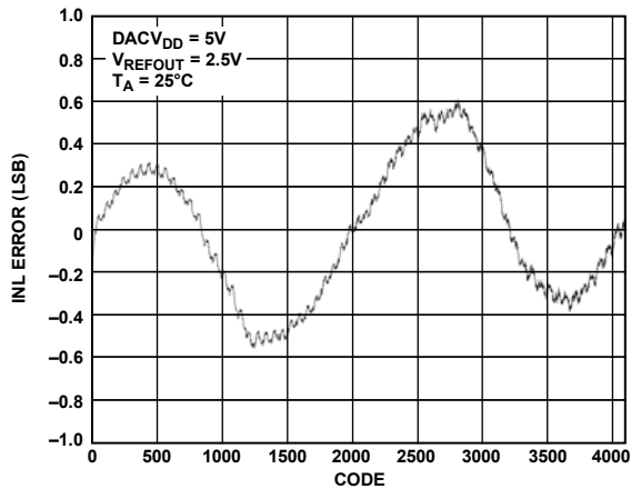
Figure 8. DAC INL, Internal Reference
