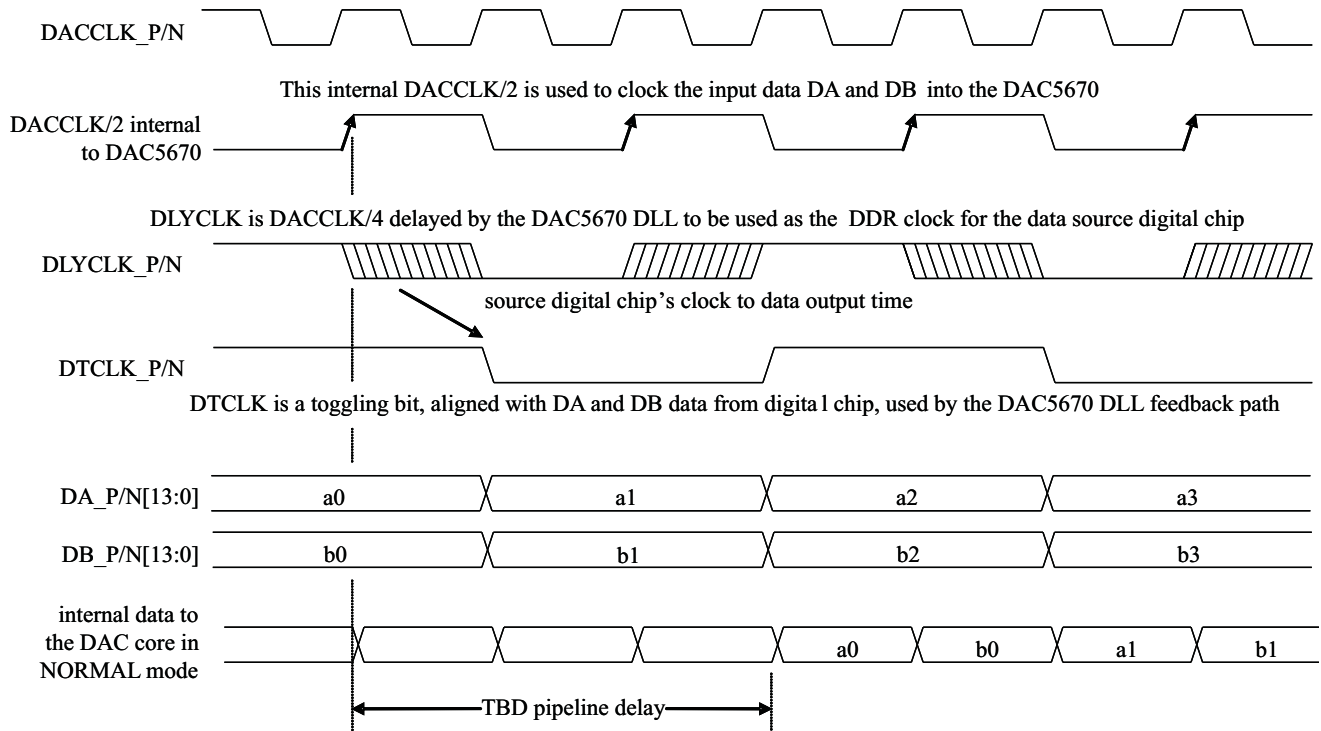
Figure 15. DLL Input Loop Functional Timing
