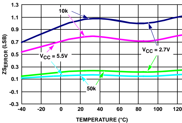
FIGURE 5. Z ERROR vs TEMPERATURE
