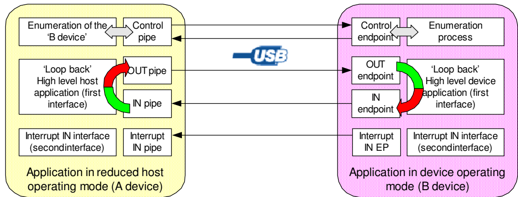
Figure 4-2. Sample application overview
