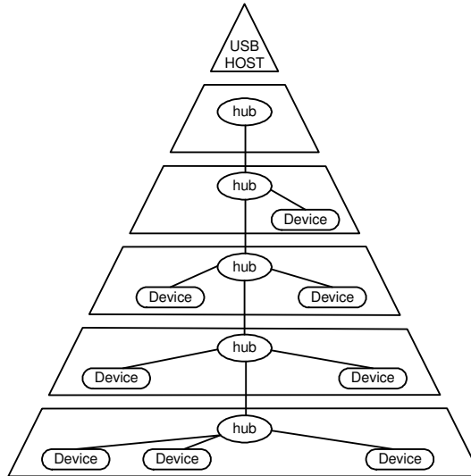
Figure 3-1. USB standard topology
