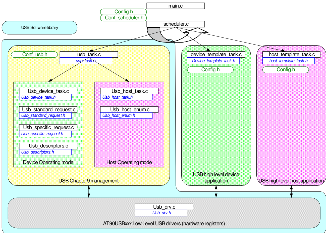
Figure 4-1. AT90USBxxx USB Firmware Architecture for dual role application
