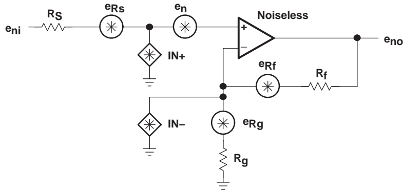
Figure 78. Noise Model
