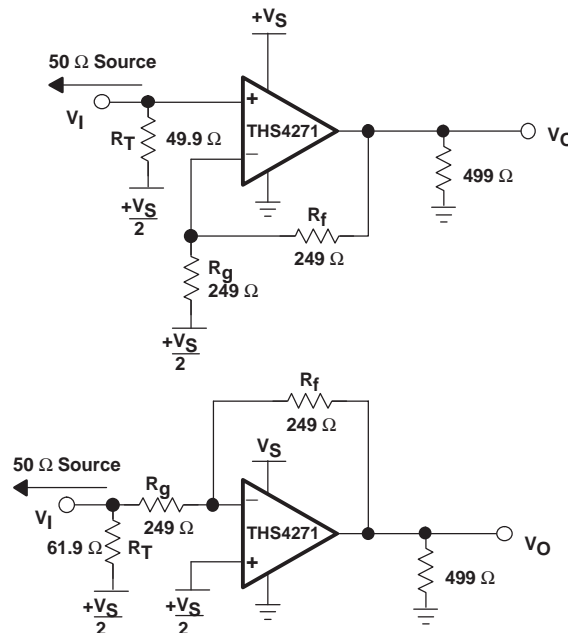
Figure 78. DC-Coupled Single Supply Operation
