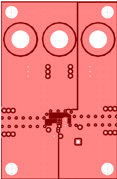
Figure 104. THS4271 Unity Gain EVM Board Layout (Third Layer, Power)
