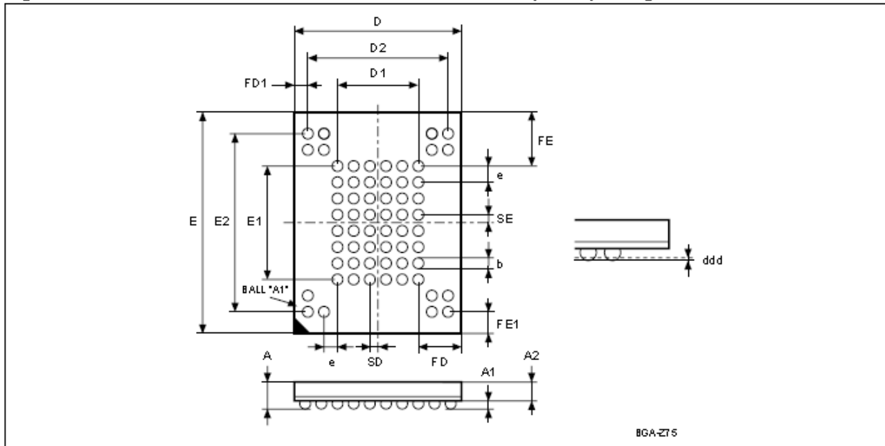
Figure 39. VFPGA63 9 x 11 x 1 mm - F6 x 8 +15, 0.80 mm pitch, package outline
