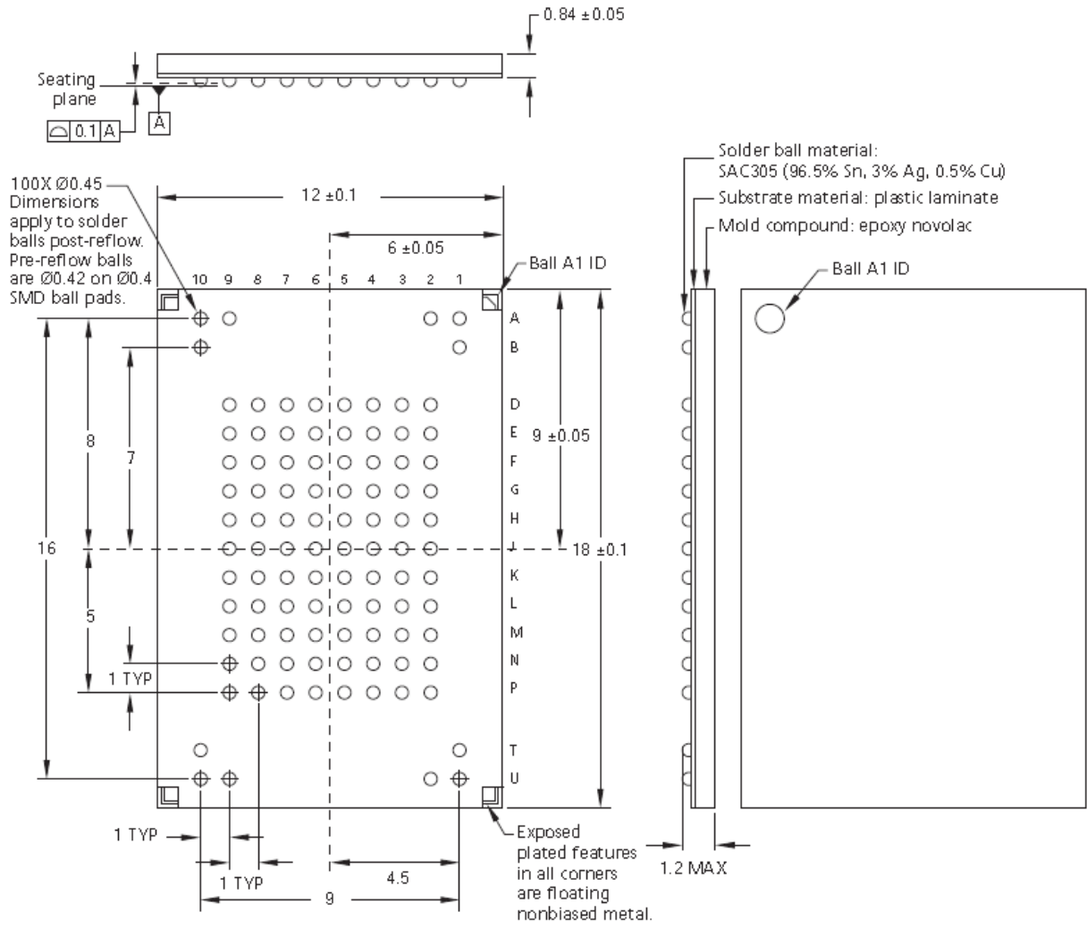
Figure 6: 100-Ball TBGA (Package Code H2), 12 x 18
