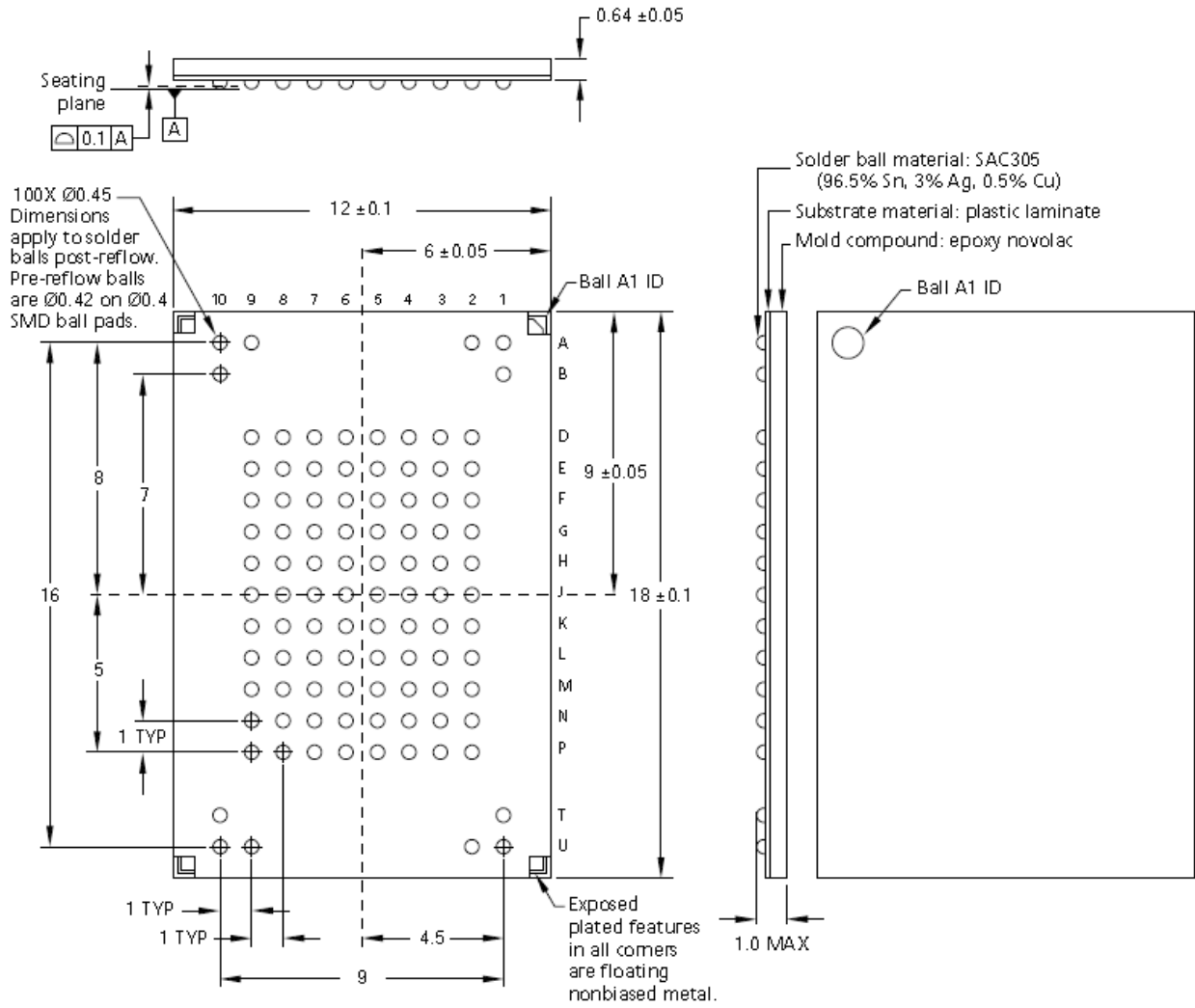
Figure 5: 100-Ball VBGA (Package Code H1), 12 × 18
