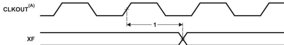
Figure 6-15. XF Timings
