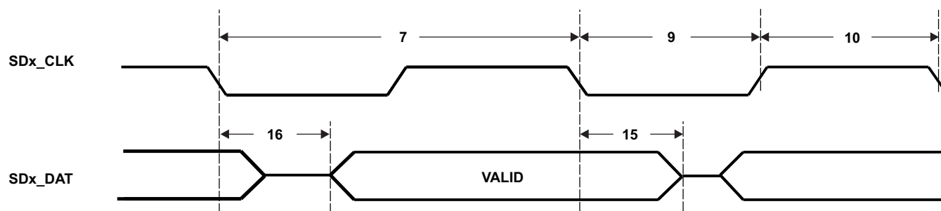
Figure 6-19. SD Data Write Timing
