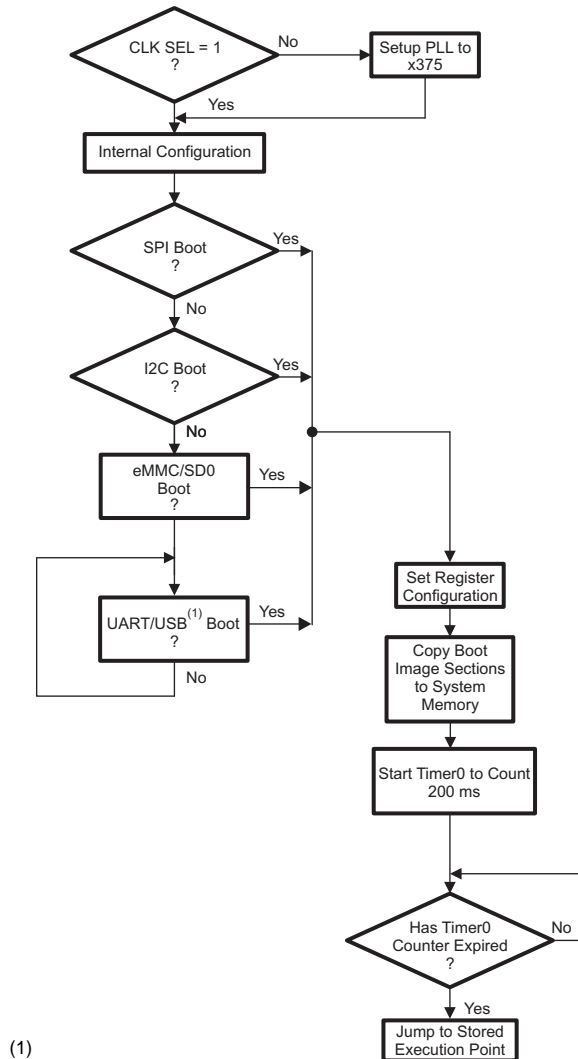
Figure 4-5. Bootloader Software Architecture
